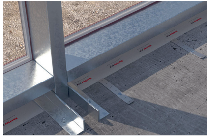
FCFcl Cavity Clad - Horizontal application
